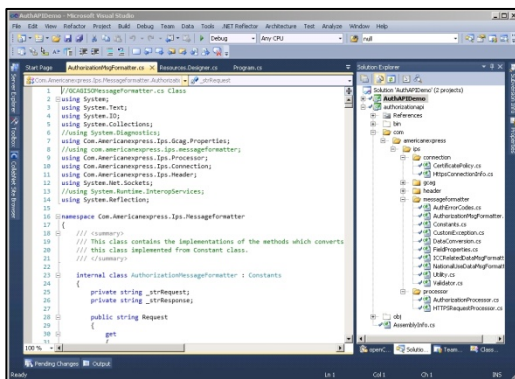
Developer Environment
